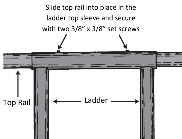
Ladder to Top Rail Assembly
